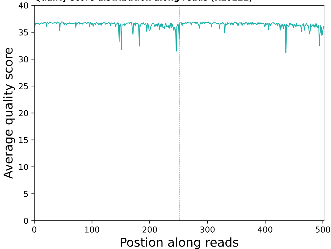
Quality score distribution along reads (R10221)
